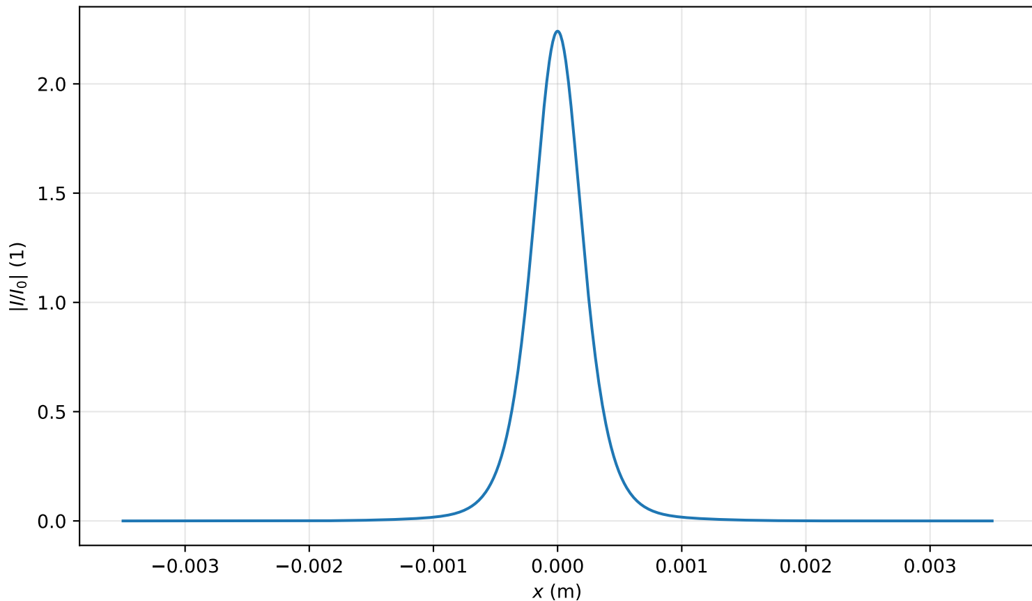
Intensity profile I(x, y = 0, z = 2.229m)/I_0 , P_{in}=1.0P_{cr} , artificial time
